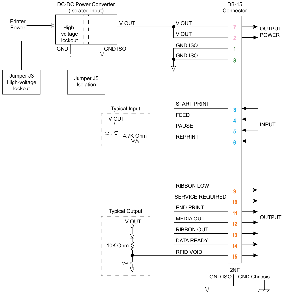
Figure 10 External Pinouts
